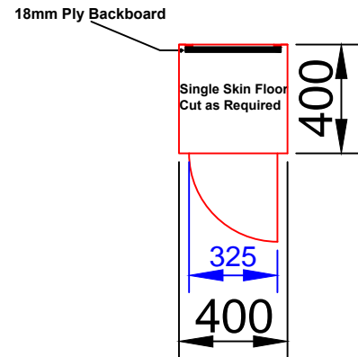
ENCLOSURE PLAN VIEW 1
